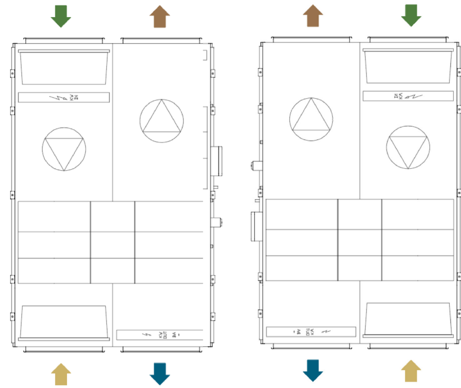
Left-hand version
