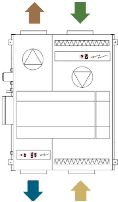
Right-hand version
