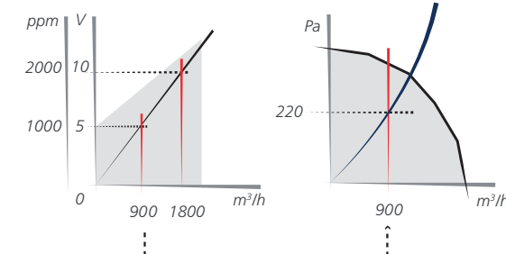
Demand control
