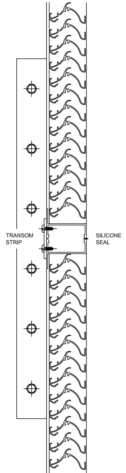
TRANSOM DETAILS
