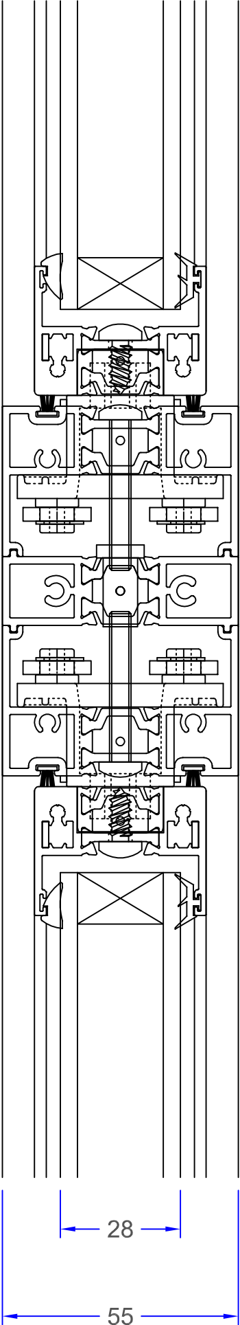
Self Mullion (Double Panel)
