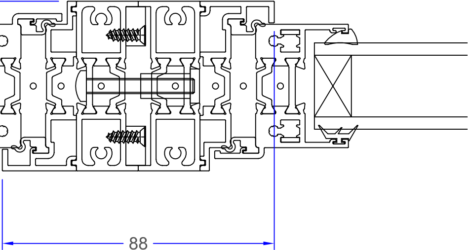
Transom Joint (Multiple Panel)
