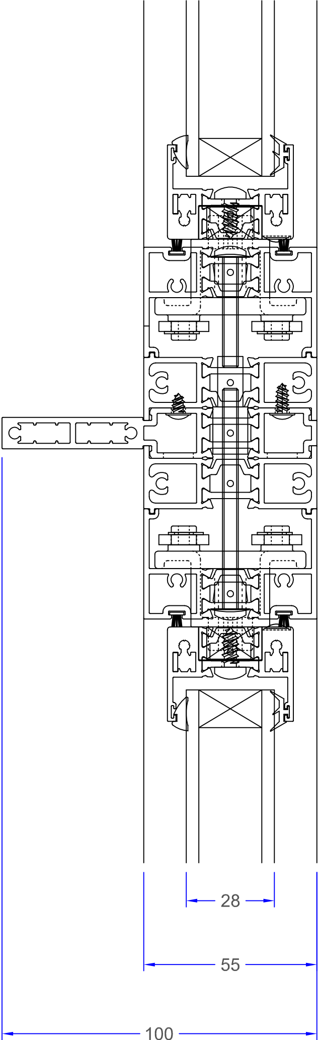
Loose Mullion (Multiple Panels)
