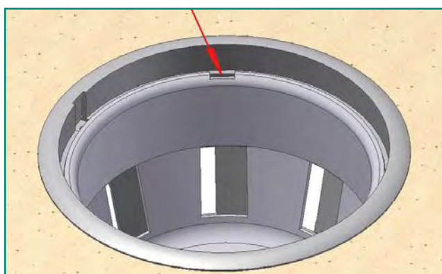
Figure 5: Install the damper and rotate until correct dovetail position is found
