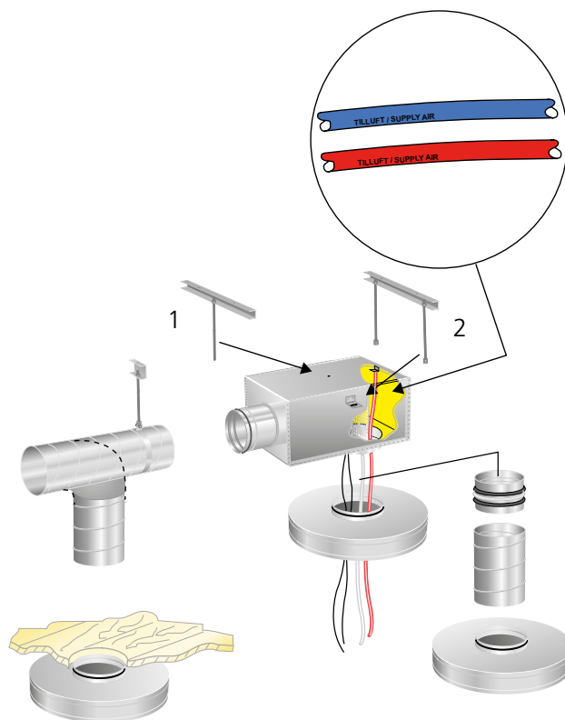
Figur 1. Montering. Innregulering.
