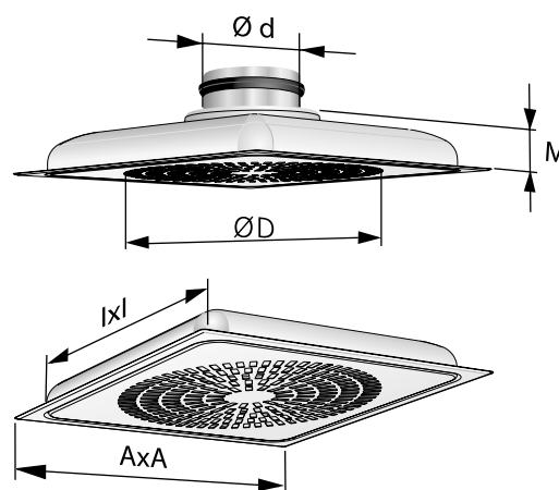
Figur 5. LOCKZONE Ceiling.
