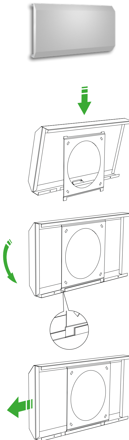
Figur 1. Montering.
