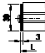
Two-slot diffuser VZ-41-2
