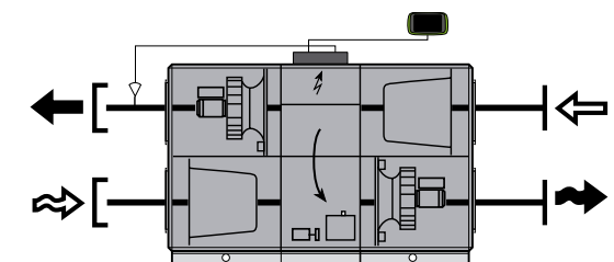
Left-hand version
