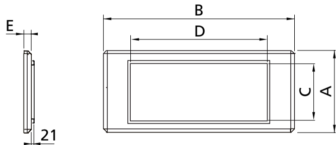
C x D correspond aux connection dimensions de la gaine
