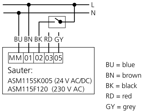
Figure 5. Wiring diagram for Sauter, 2 point regulation.
