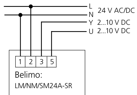
Figure 10. Wiring diagram for Belimo, 2-10 V stepless / modulating regulation.
