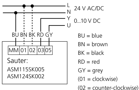
Figure 7. Wiring diagram for Sauter, 0-10 V stepless/modulating regulation.
